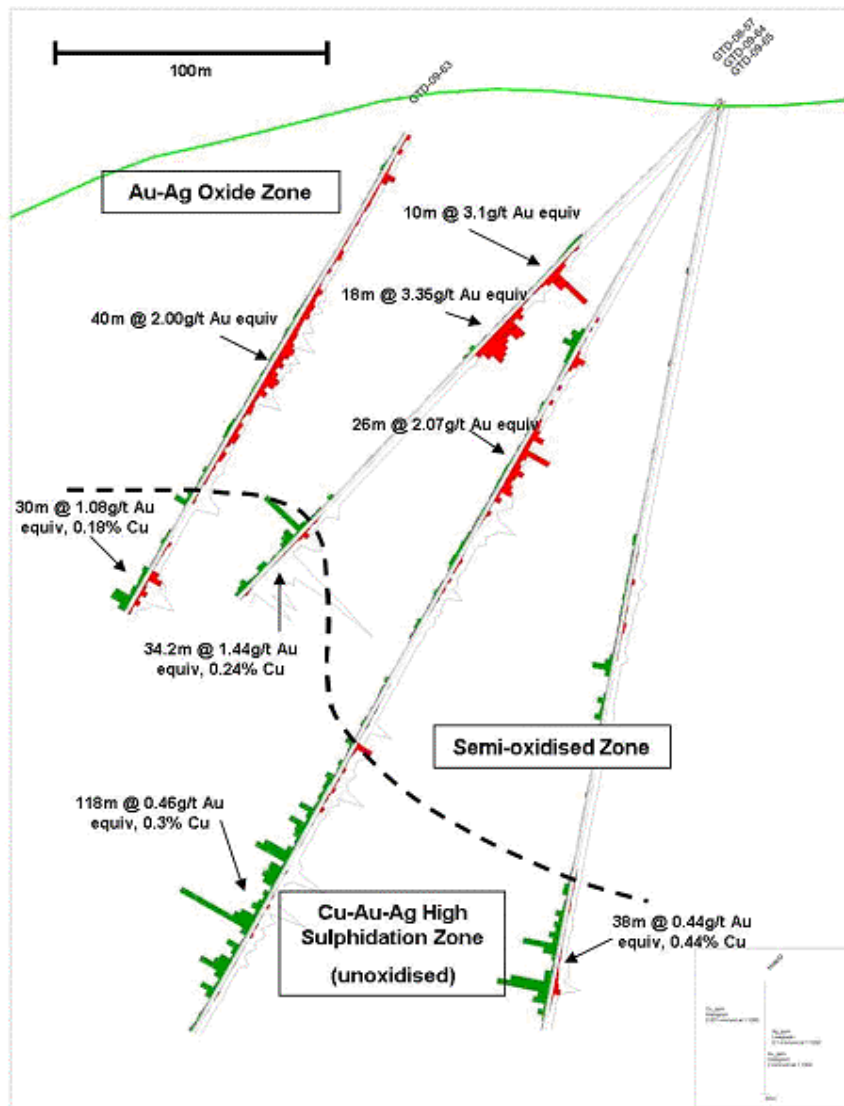
Cross section through the central Zone B drilling area showing high grade domains in the oxide gold-silver zone, surrounded by lower grade haloes; and overlying a relatively shallow significant copper-gold-silver high sulphidation zone. This zone has not been tested by any deep drilling.
