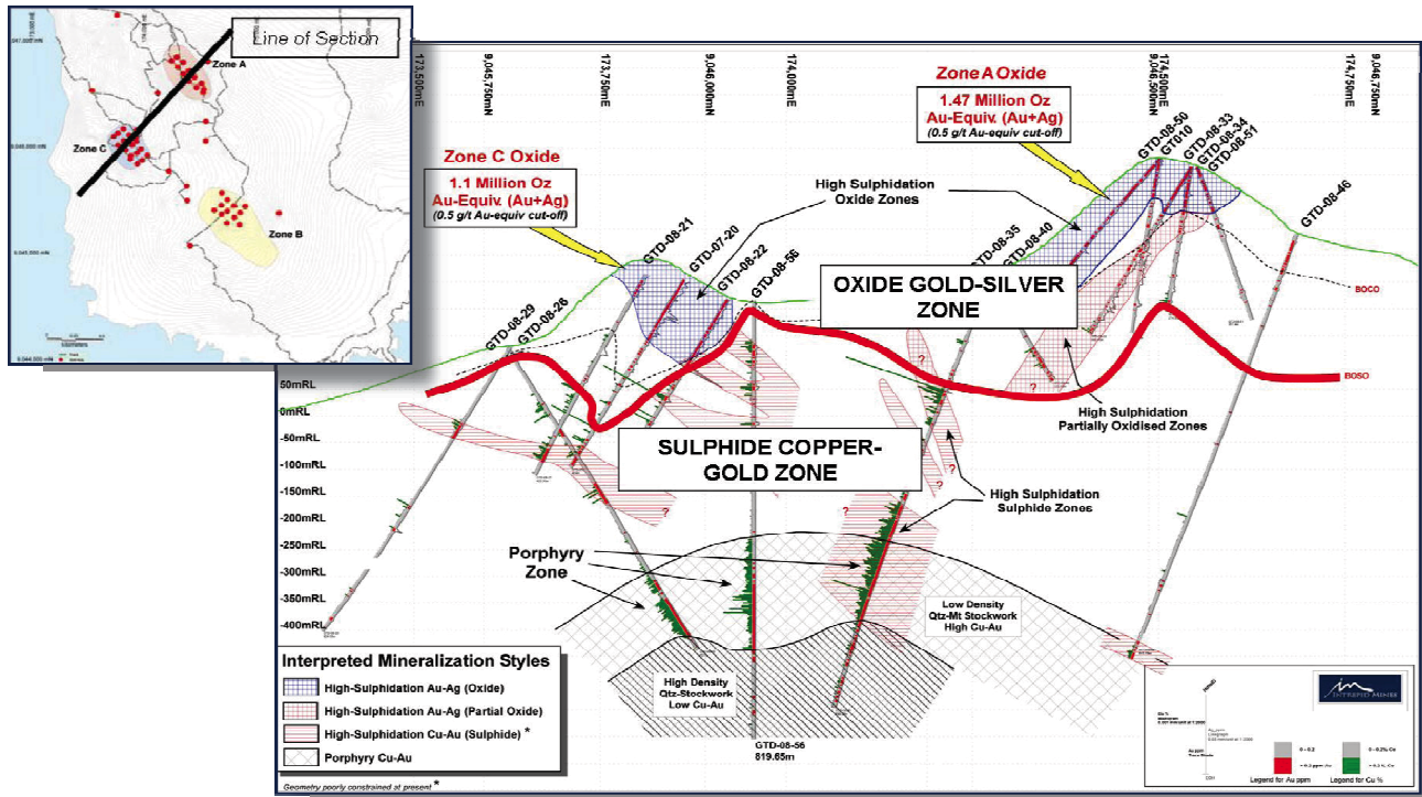
Figure A – cross section through the Tujuh Bukit mineralisation showing the oxide and sulphide zones.
