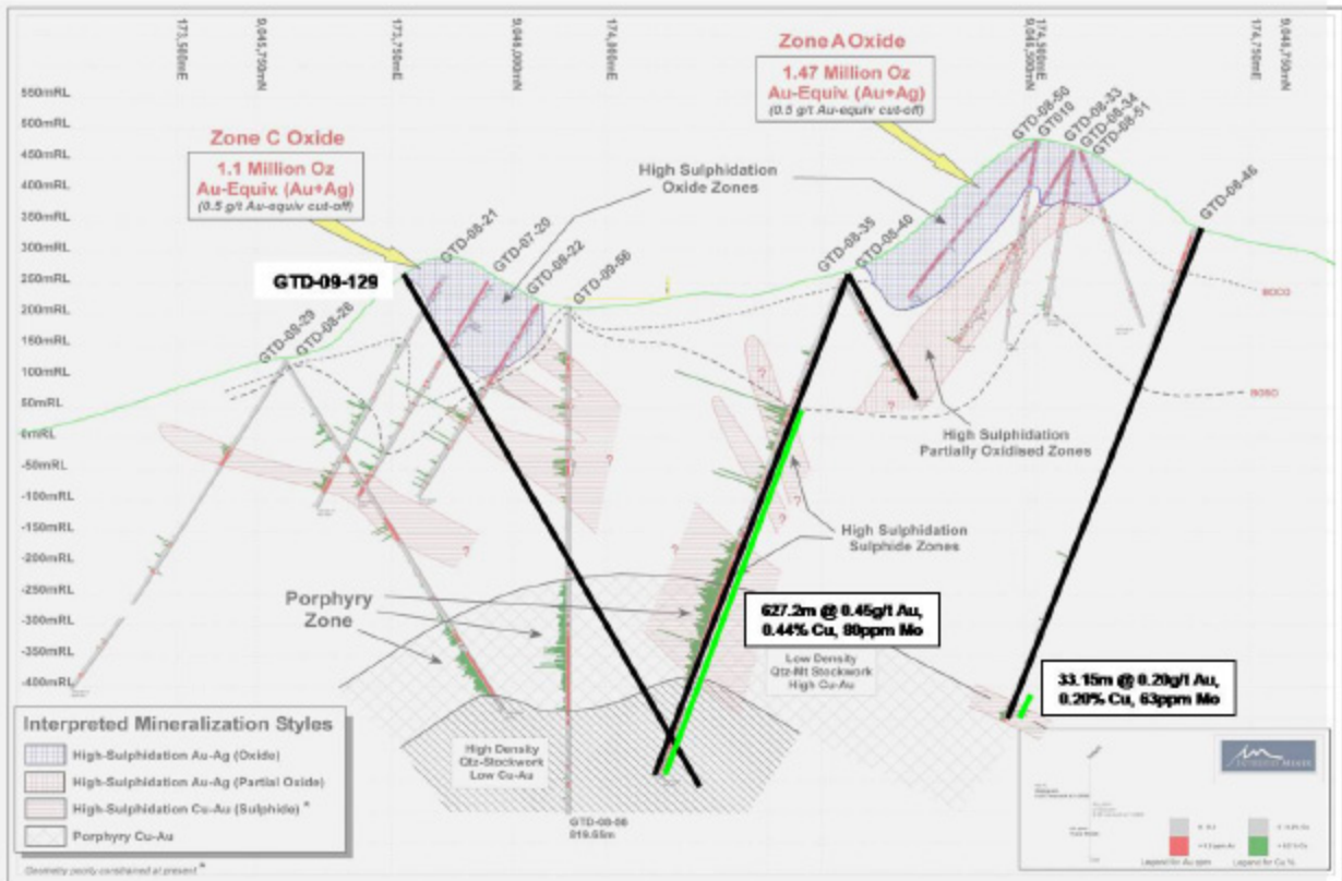
Drill Section 1 – Drill holes shown in bold occur on this section. Hole GTD-09-129 has been drilled but assays have not yet been returned.
