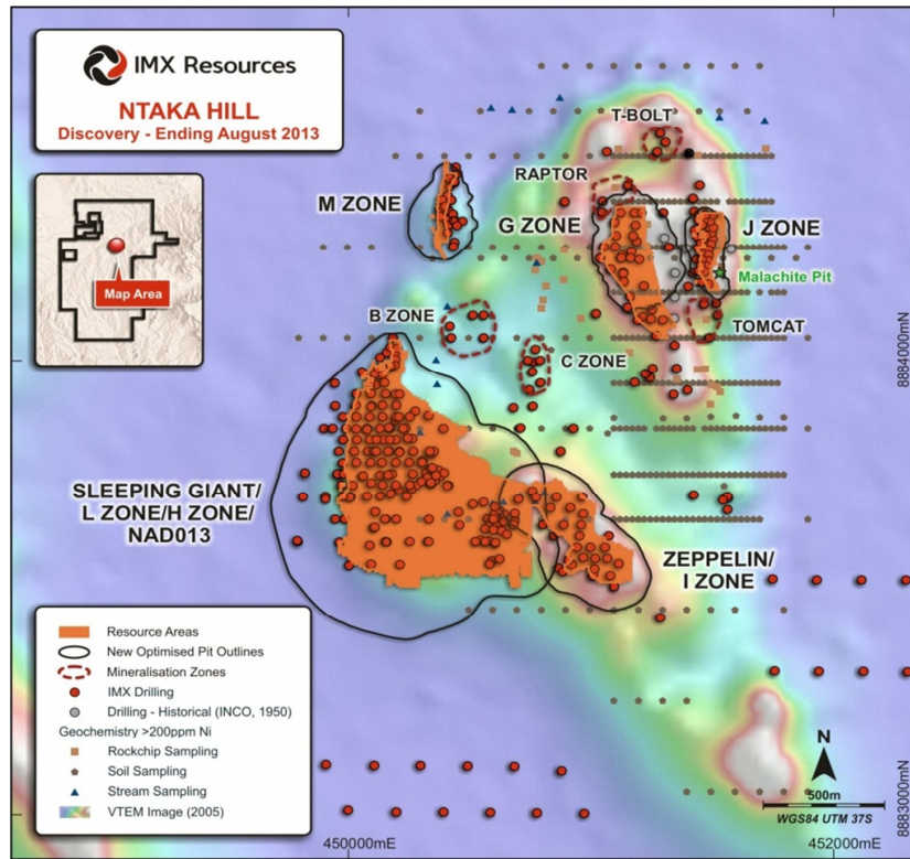
Figure 2: Ntaka Hill General View (2013)
