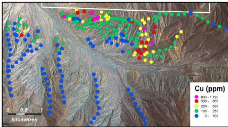
Talus Fines Copper Anomalies at Surface
