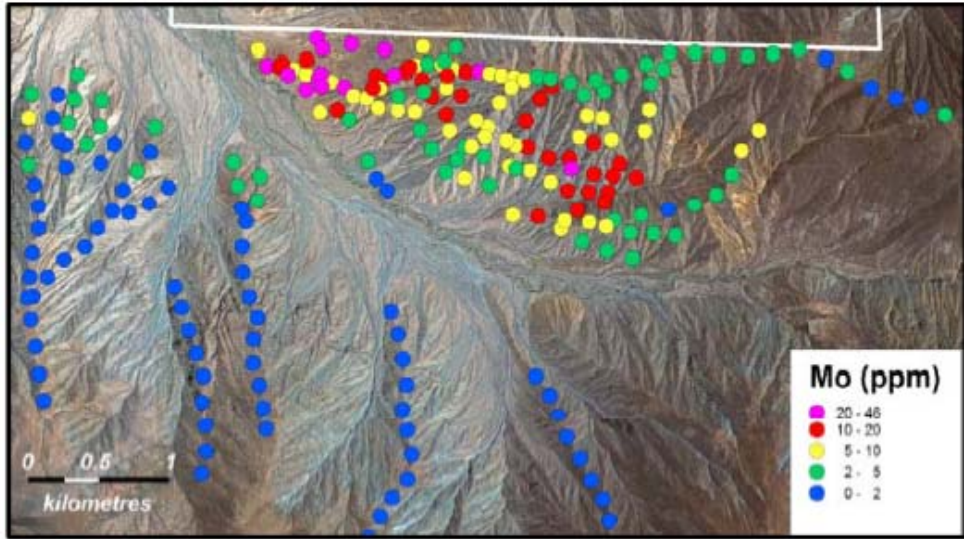
Talus Fines Molybdenum Anomalies at Surface
