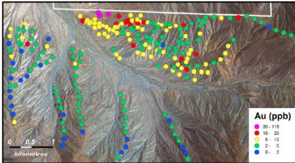
Talus Fines Gold Anomalies at Surface
