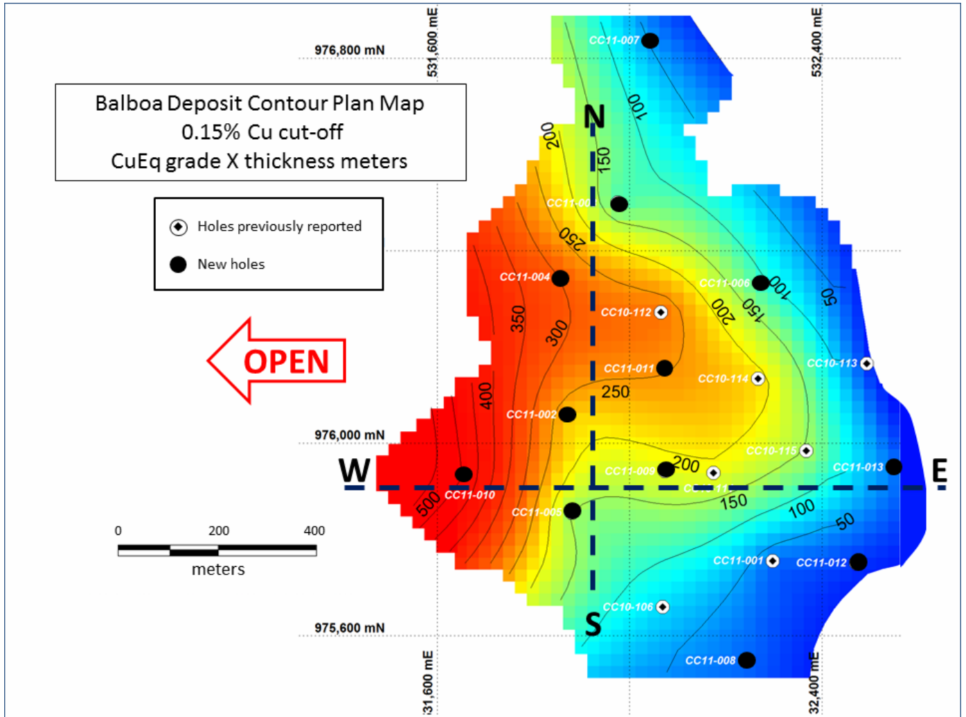
Figure 1: Plan Map- Balboa Discovery May 2011
