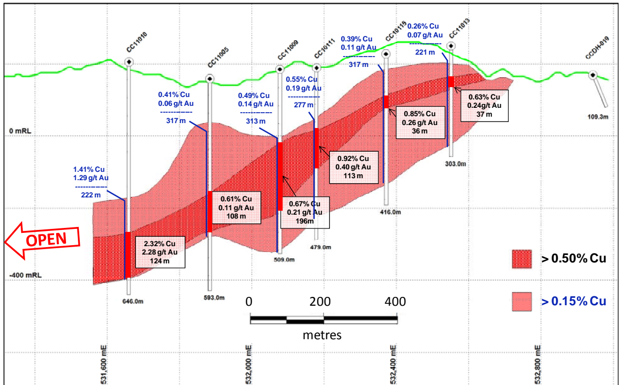
Figure 3: Section South North – Balboa Discovery May 2011
