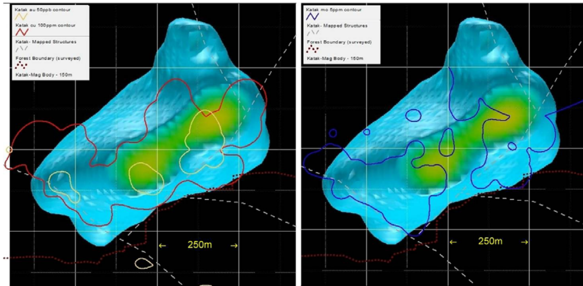
Images showing the 3-D model of the Katak heli-mag anomaly with contours from surface geochemistry – red = copper, yellow = gold, blue = molybdenum. The magnetic anomaly is coincident with mapped diorite and soil geochemical anomalies.
