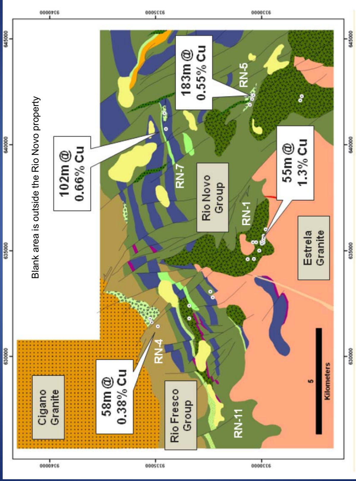
Figure 2: Southern Portion of Rio Novo Geology & Selected Intersections
