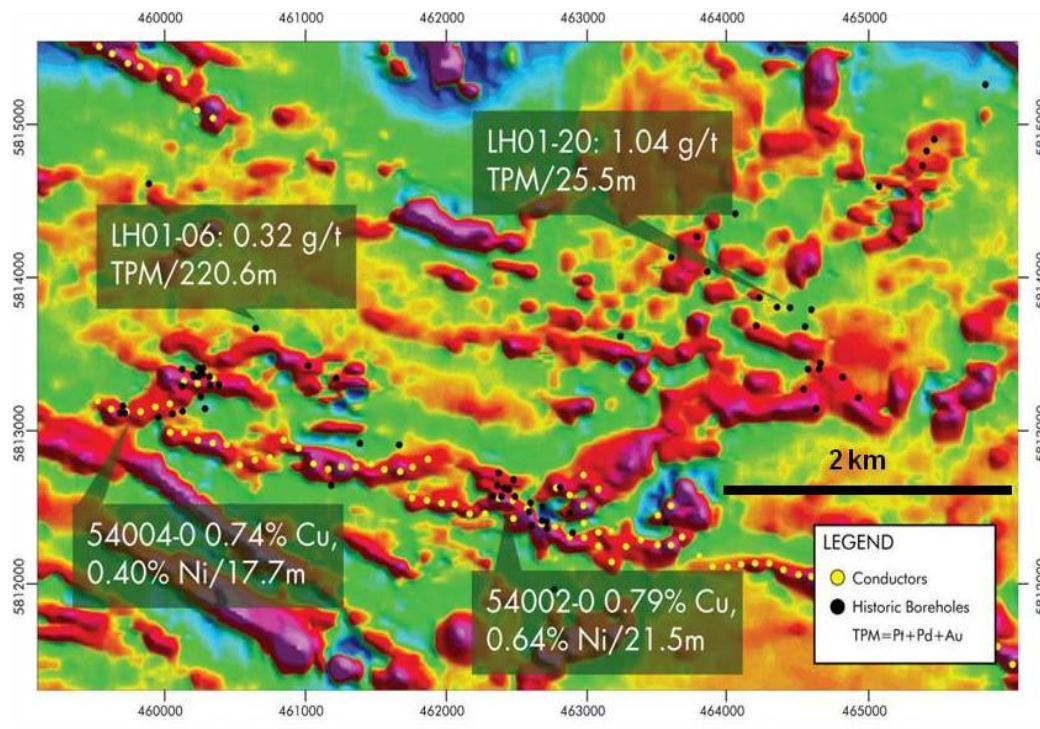
Figure 3 - Detail Area Magnetics and Electromagnetic Conductors
