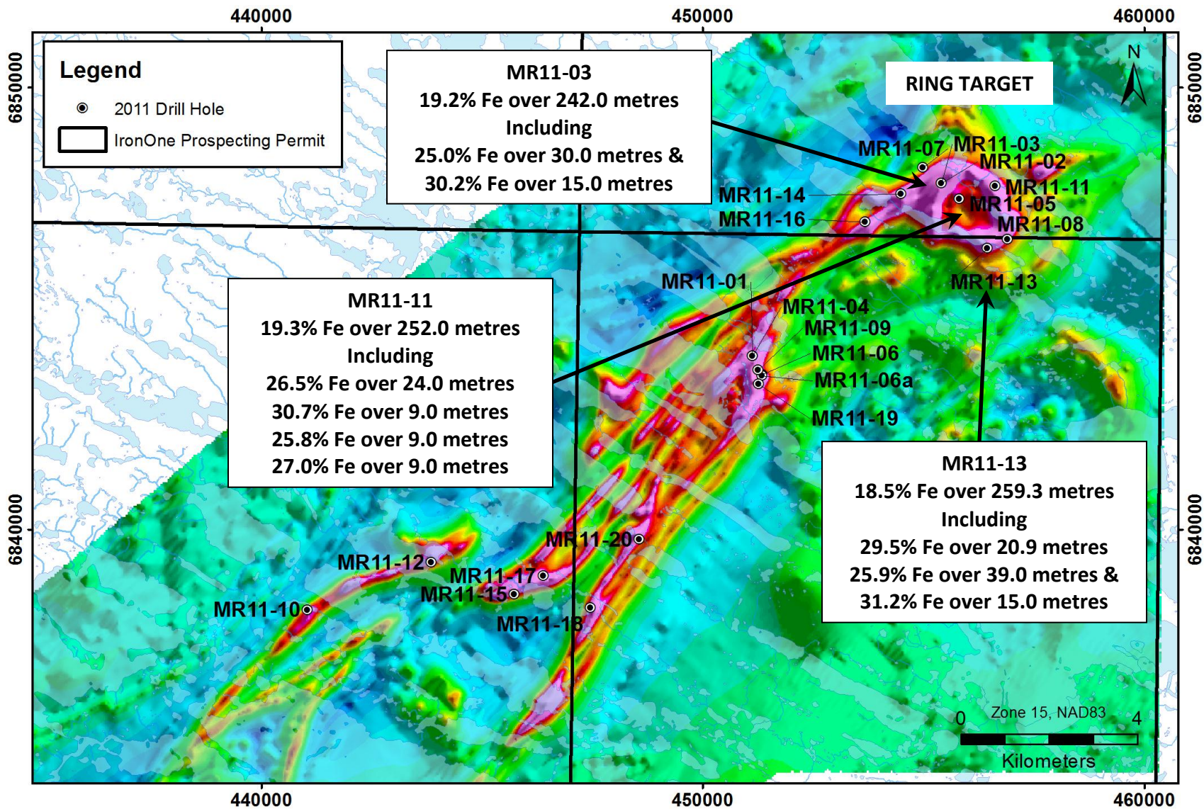
Figure: Drill Hole Location Plan Map, Maguse River Iron project, southern Nunavut. (Background – airborne Magnetic Survey (Total Magnetic Intensity (TMI))).
