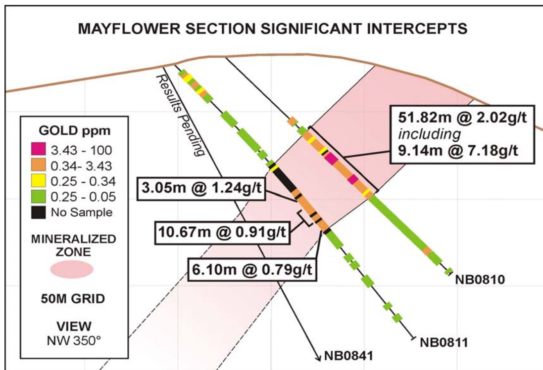
Figure 1. Section through holes NB08-10, 11 and 41, illustrating the broad southerly dipping mineralized zone.
