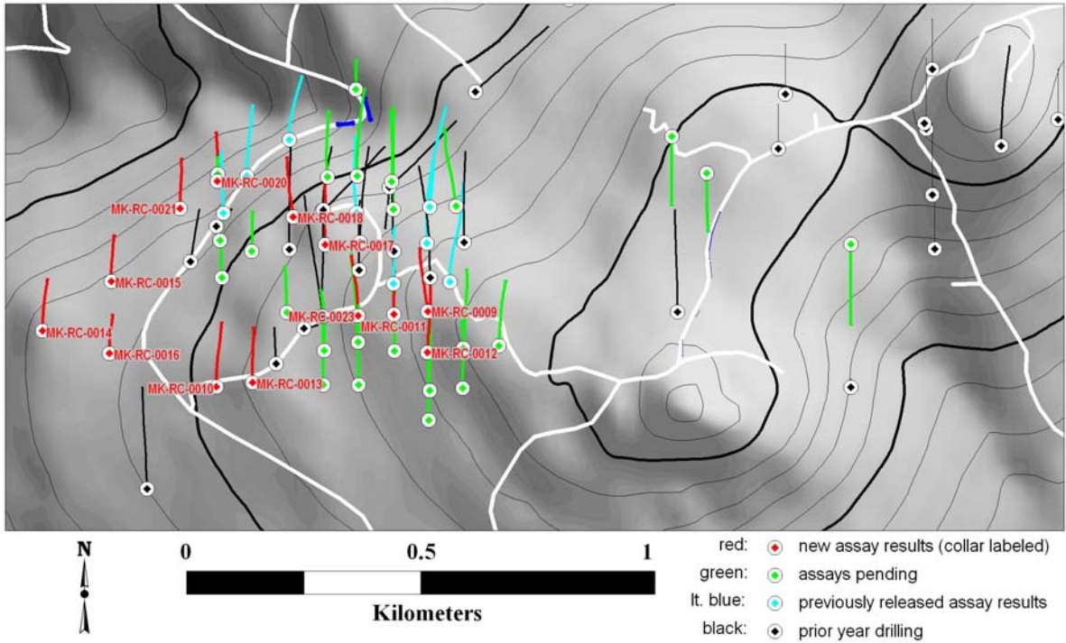
Figure 1 Livengood drill hole plan map. (The 14 new drill holes for which data is reported in this release are shown in red.)
