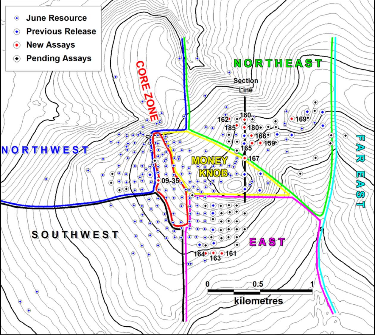
Figure 2: Location of new assays from Livengood
