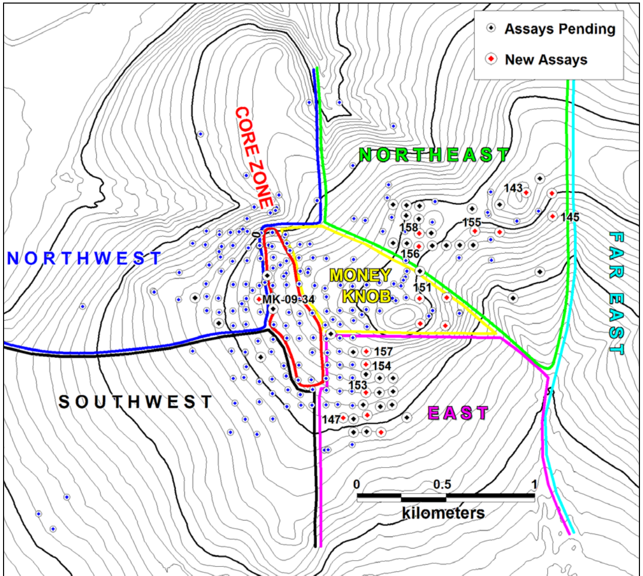
Figure 1: Plan showing Summer 2009 holes completed to date (143-195) and those for which assays are reported in this news release. The focus of the summer program is the expansion of the deposit in the East and Northeast areas with preliminary testing of the Far East. The results reported here confirm the continuity of significant mineralization over a strike length of 1000 metres in the Northeast sector.
