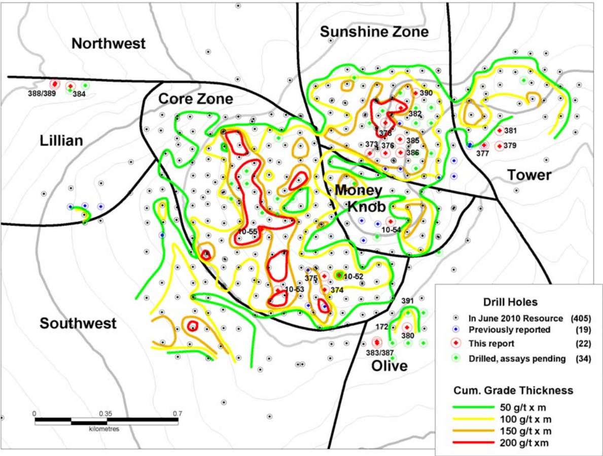
Figure 1: Locations of new assay results and current cumulative grade thickness map. Grade thickness contours are plotted relative to the collar locations shown.
