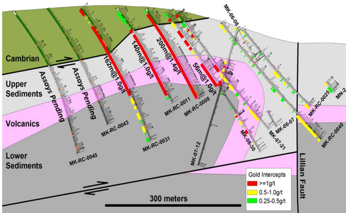
Section 428925 illustrating the general geology of Livengood deposit and distribution of gold mineralization. Histogram on the right side of the drill traces reflect the arsenic content which has a high correlation to gold (note pending holes).
