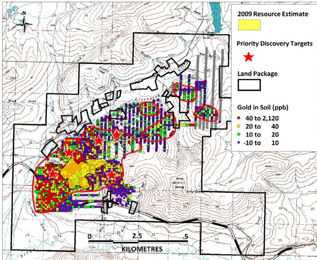
Figure 2 Livengood Amended Land Map illustrating gold in soil and priority discovery targets.
