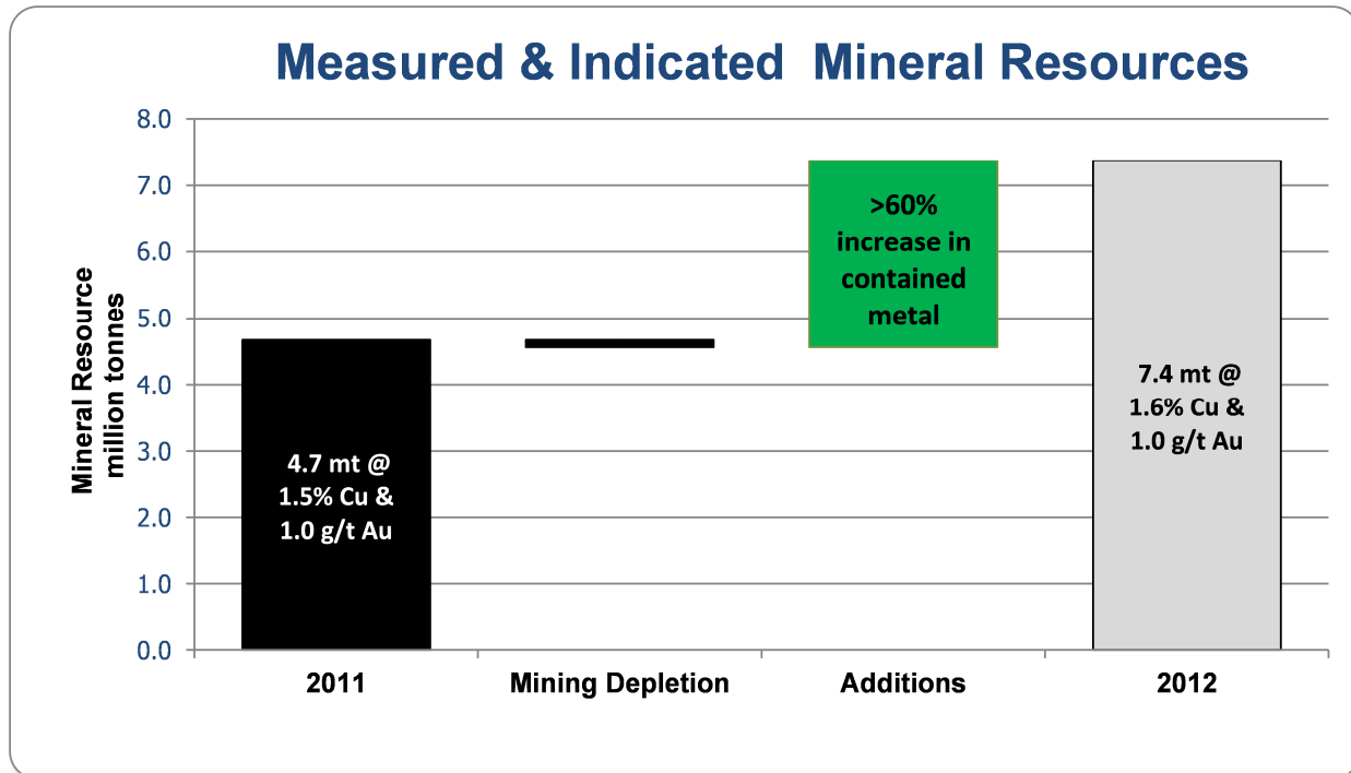
Figure 2 –Kulthor Measured & Indicated Mineral Resource – changes: 2011–2012.
