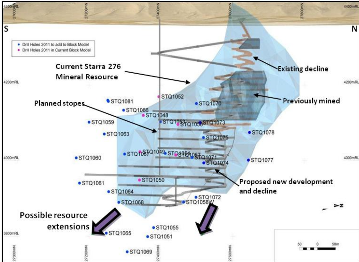
Figure 2. Starra 276 Long Section Looking West
