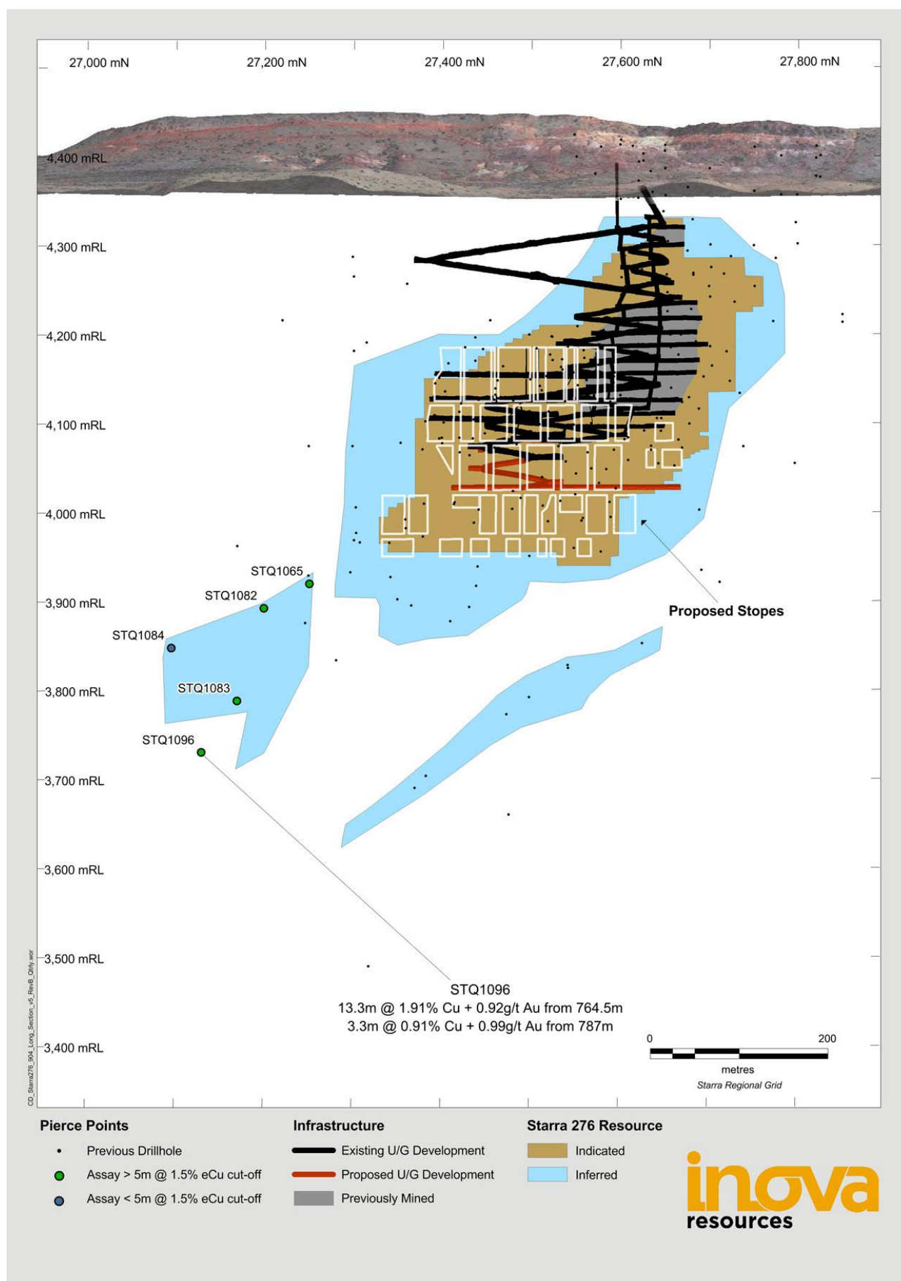
FIGURE 2. STARRA 276 LONG SECTION – SHOWING LOCATION OF HOLE STQ1096
