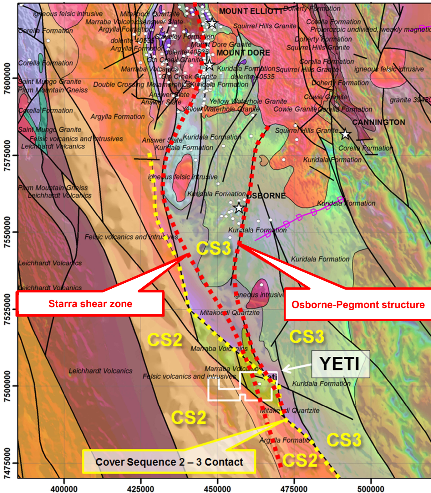
Figure 6. Yeti - Regional Geological Features
