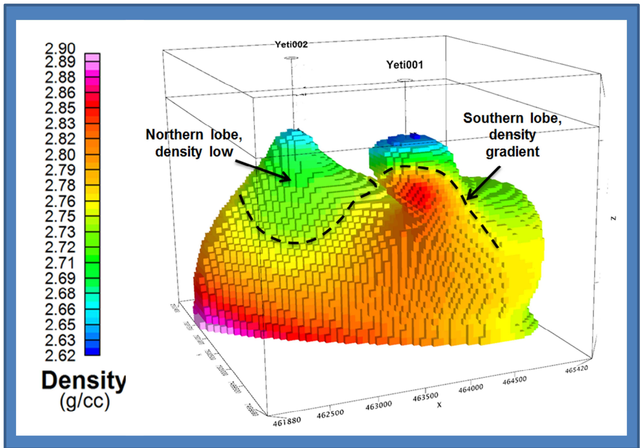
Figure 3. Yeti – 3D Perspective view of the most magnetic portion of the Yeti Anomaly
