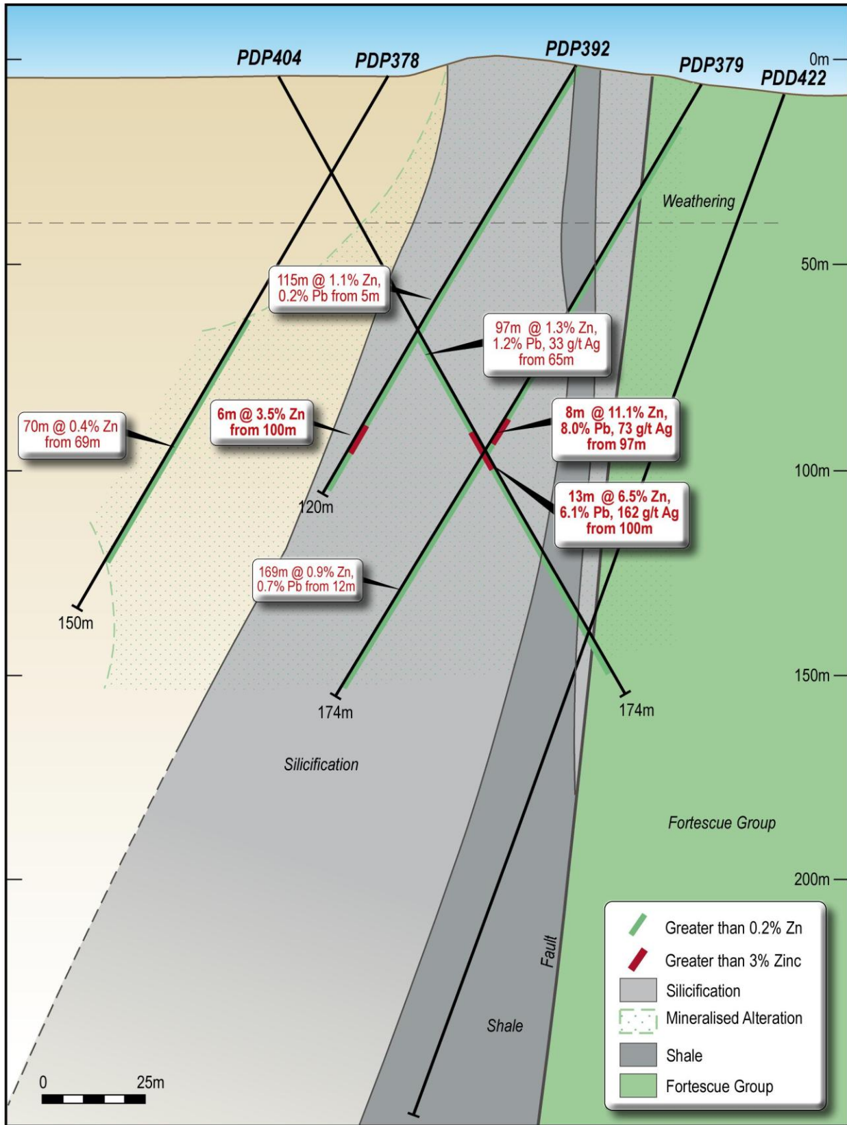
Figure 3. Wolf prospect Cross-section (northern portion on PDP404, looking northwest).
