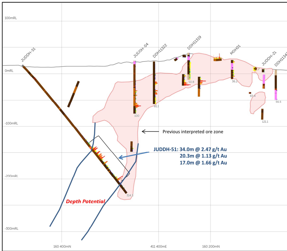
Bau Gold Project Jugan Deposit Section Looking Northeast
