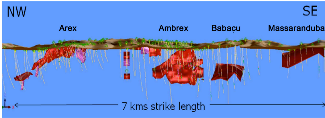
Figure 1. Long Section of the northern sector of the Aripuanã Massif Sulphide District
