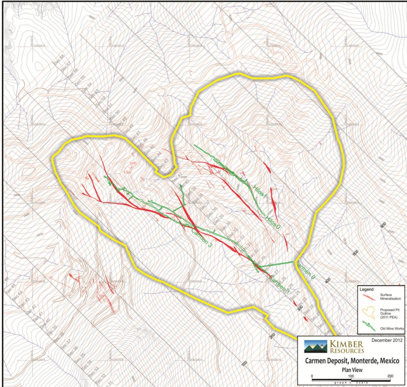
Figure 1: Carmen Deposit Showing Historic Workings: Carmen and Hilos Structures
