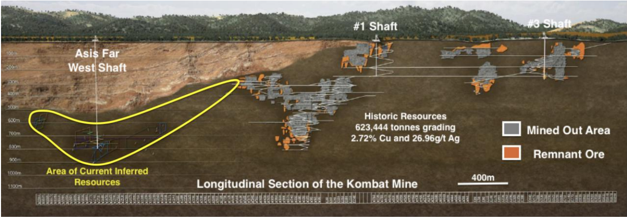
Figure 1: Longitudinal Section Identifying Area of Current Inferred Resources.
