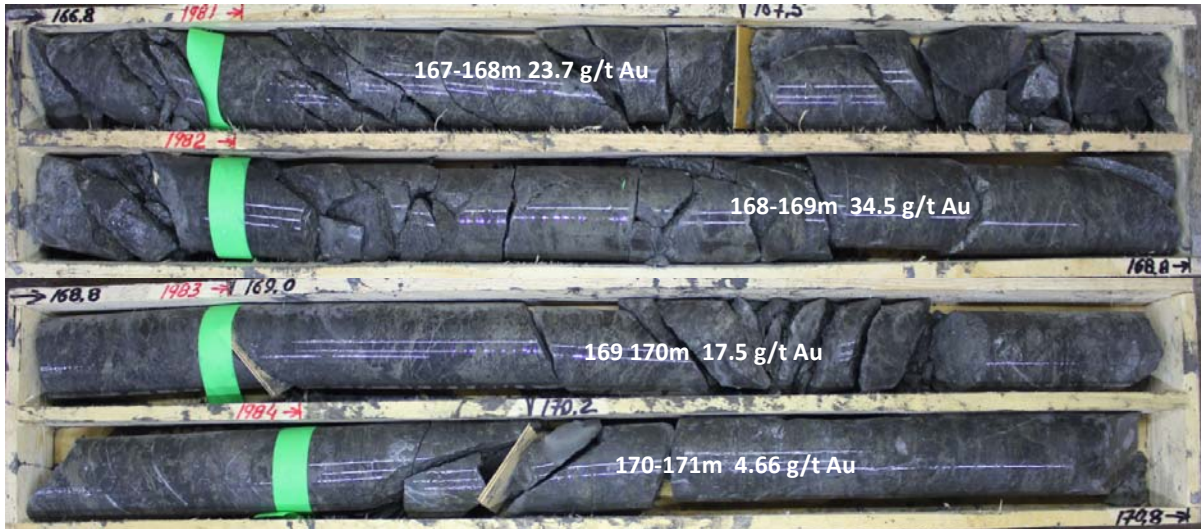
Mineralized drill core TBL East Zone DDH EZ-1-17, 167-171m, pervasive silica-tourmaline-pyrite altered meta-sediment.
