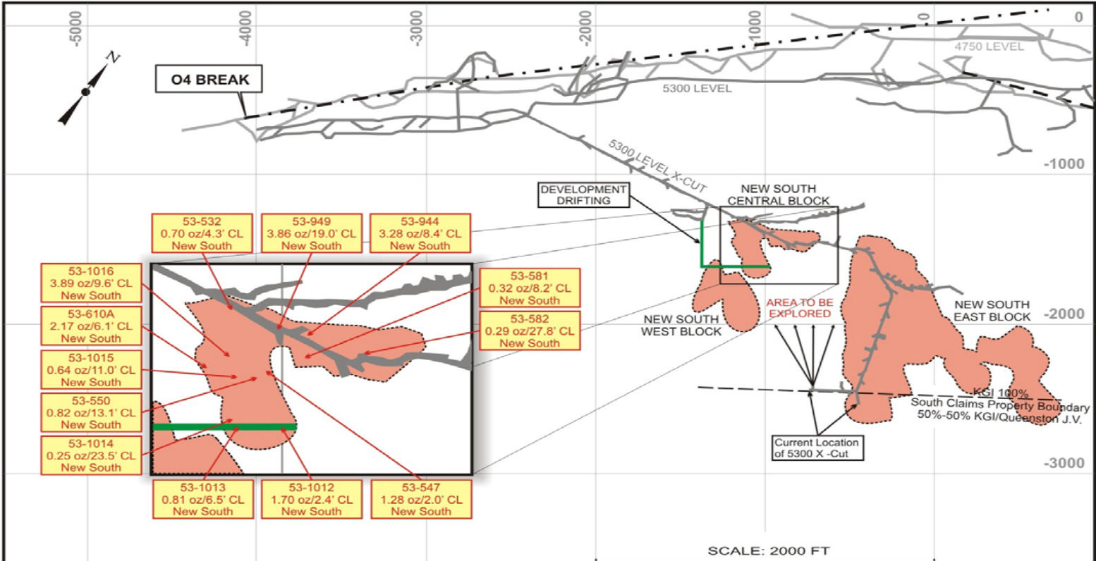
PLAN VIEW OF RECENT DRILLING SHOWING NEW SOUTH ZONE INTERSECTIONS #3 SHAFT AREA, KIRKLAND LAKE GOLD INC, KIRKLAND LAKE, ONTARIO
