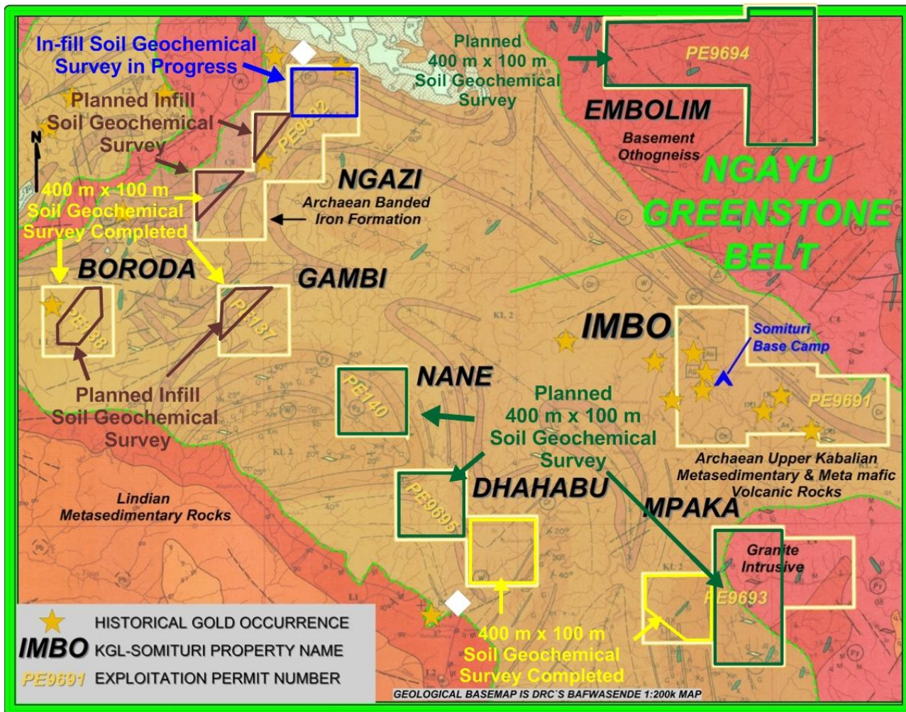
Figure 1. Geological map illustrating the Somituri PEs and status of soil geochemical surveys on all PEs except Imbo.
