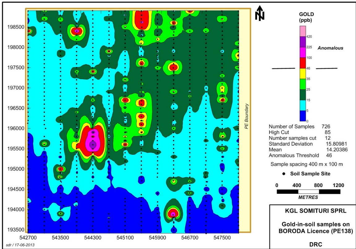
Figure 2. Map of contoured gold geochemical values, Boroda Licence, Somituri Project, DRC.
