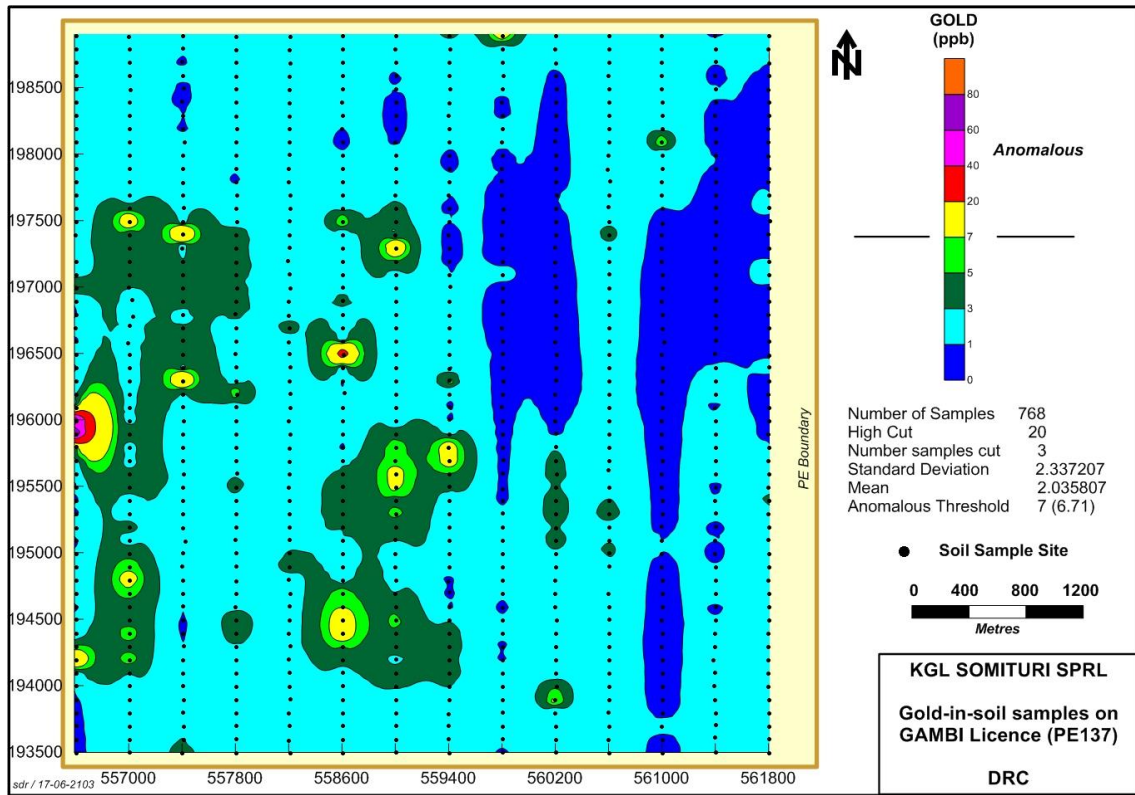
Figure 3. Map of contoured gold geochemical values, Gambi Licence, Somituri Project, DRC.
