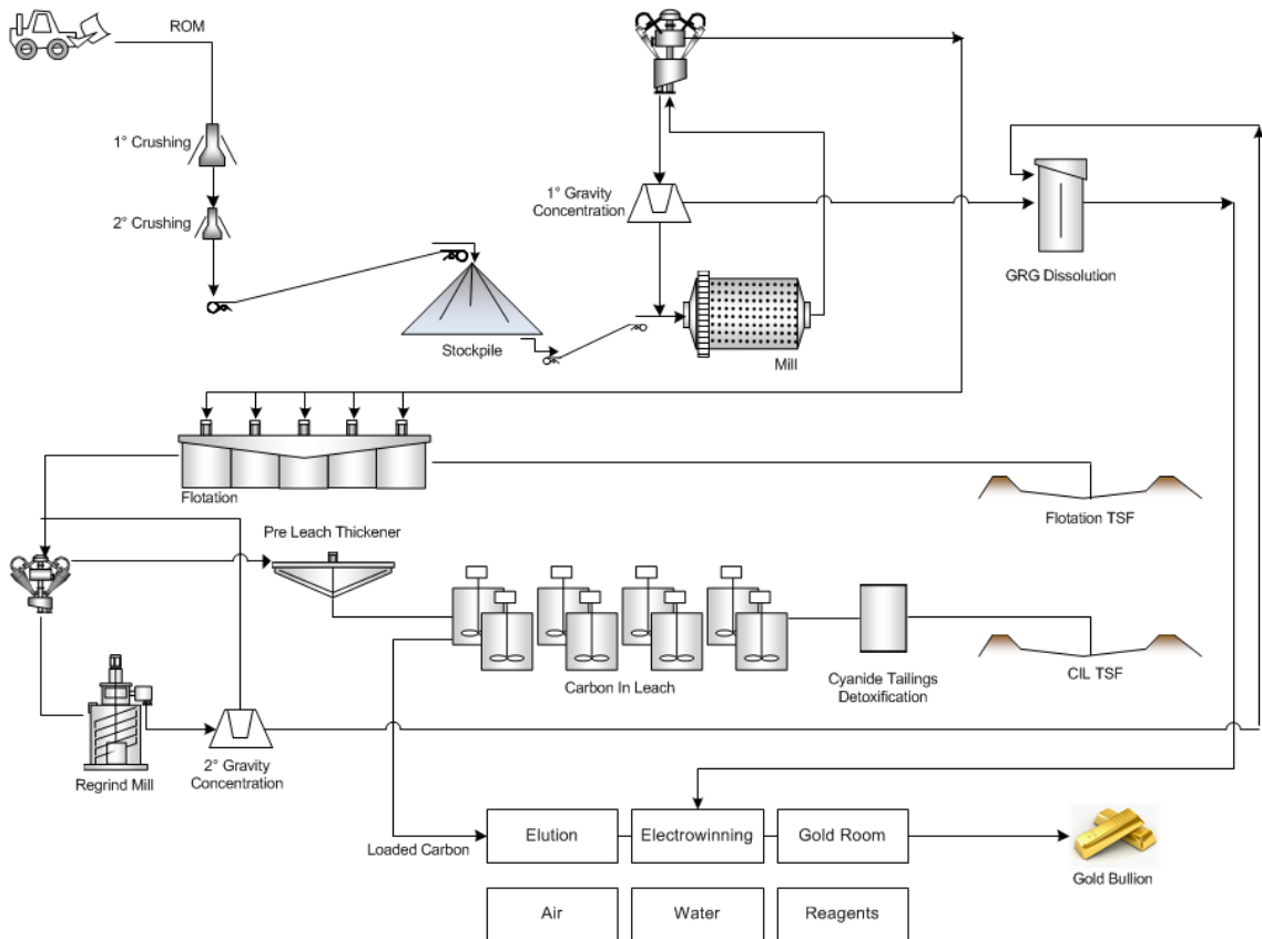
Figure 1: Final simplified flow sheet for the Esaase Gold Project
