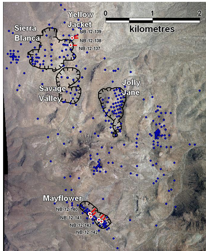
Figure 1: North Bullfrog Project area showing the location of drill holes reported in this release and mine pits outlined in the Preliminary Economic Assessment (NR 12-07, Feb. 28, 2012)
