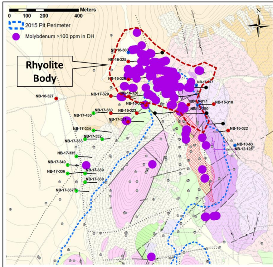
Figure 2. Map of elevated Molybdenum and Rhyolite intrusive at the north end of the Sierra Blanca-YellowJacket deposit, North Bullfrog Project
