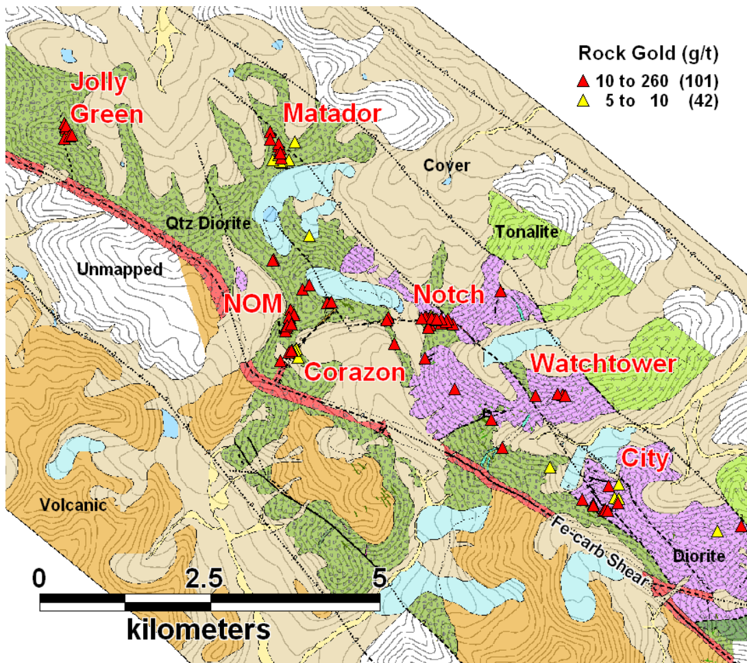
Figure 1: Geological map of the Golden Range Target showing major prospects and gold in surface rock samples.
