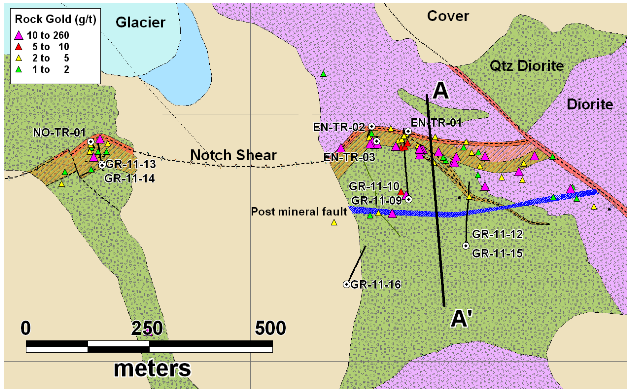
Figure 2: Geological map of the Notch Zone showing surface rock samples with drill and trench locations and traces.
