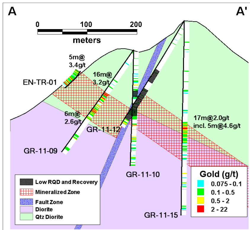
Figure 3: Geological cross section through the Notch Zone
