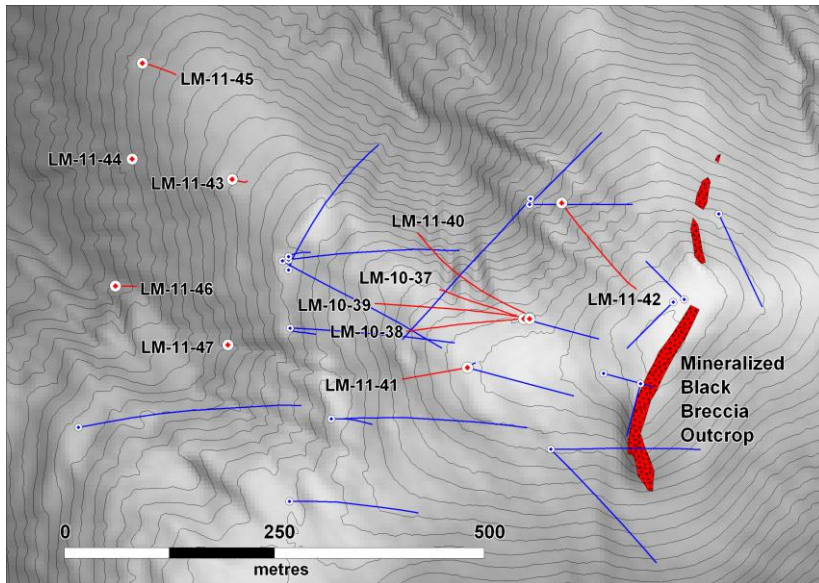
Figure 1: Map showing the locations of new core holes drilled at LMS in 2011. These holes represent a significant expansion of the area of mineralization and confirm the structural continuity of the deposit.
