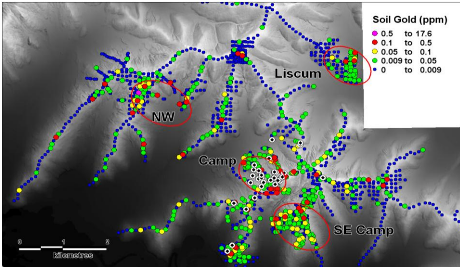
Figure 2: Gold in soil anomaly map for LMS property
