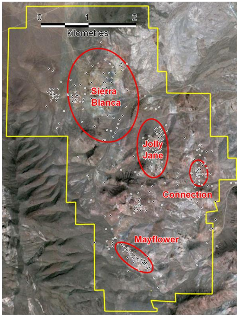
Figure 1: Corvus land position at North Bullfrog showing the Mayflower Resource Area, and the Other Resource Areas. Drill collar locations are shown for reference.
