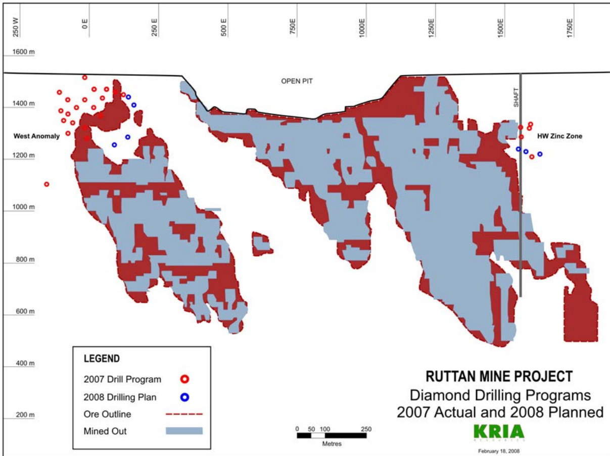
Figure 2 – Ruttan Longitudinal Section of Drilling Completed and Underway
