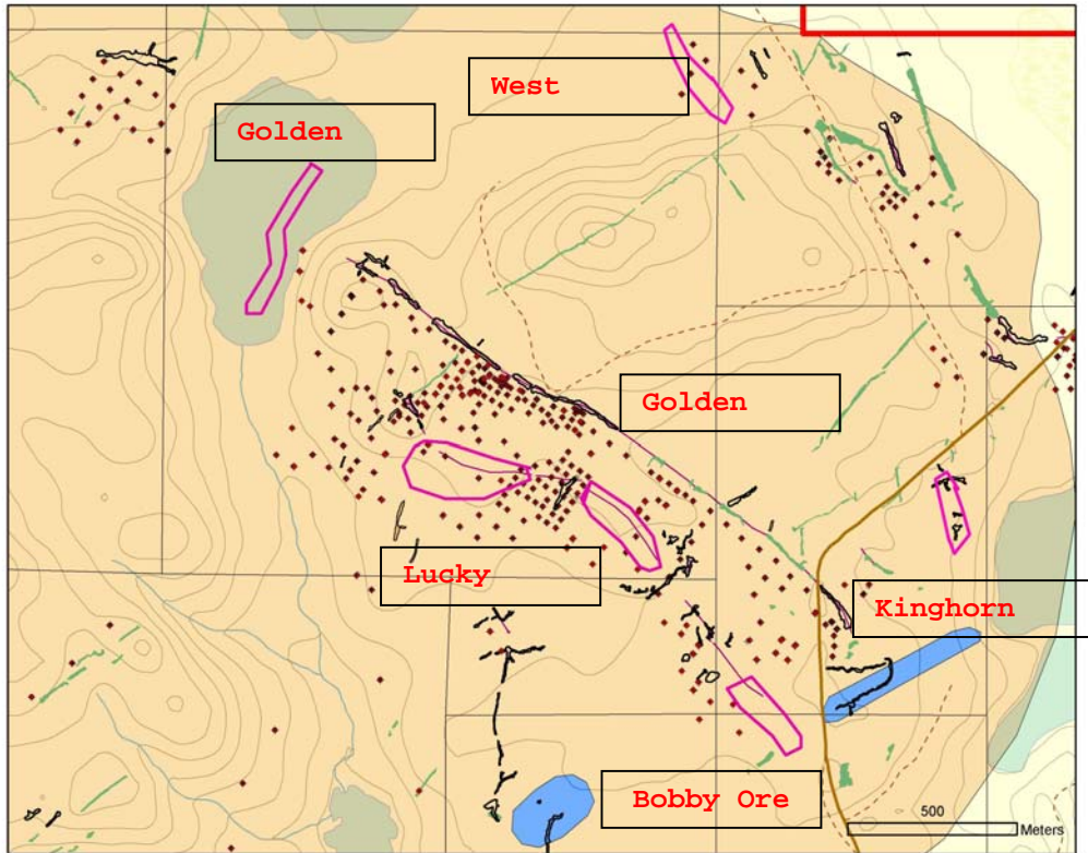
Winter 2010 proposed drilling areas, Hercules Project. Individual target areas are outlined in magenta.
