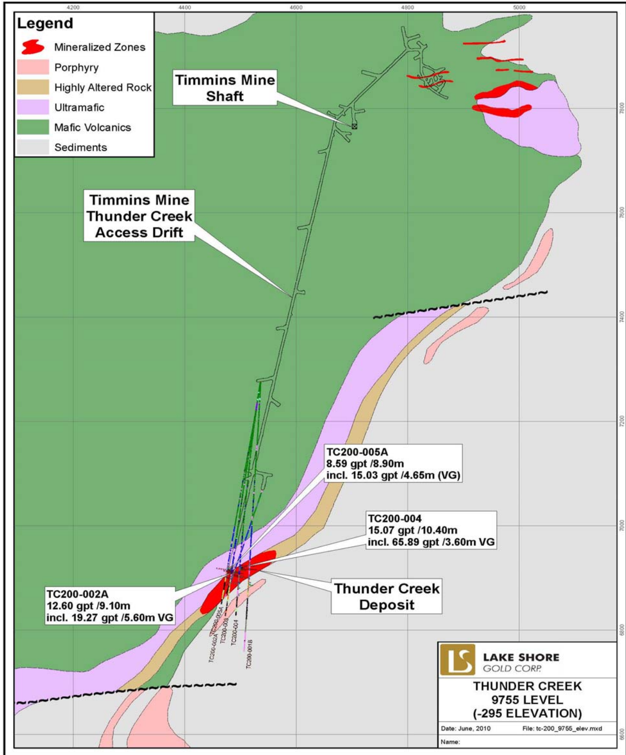
Figure 1. Plan View
