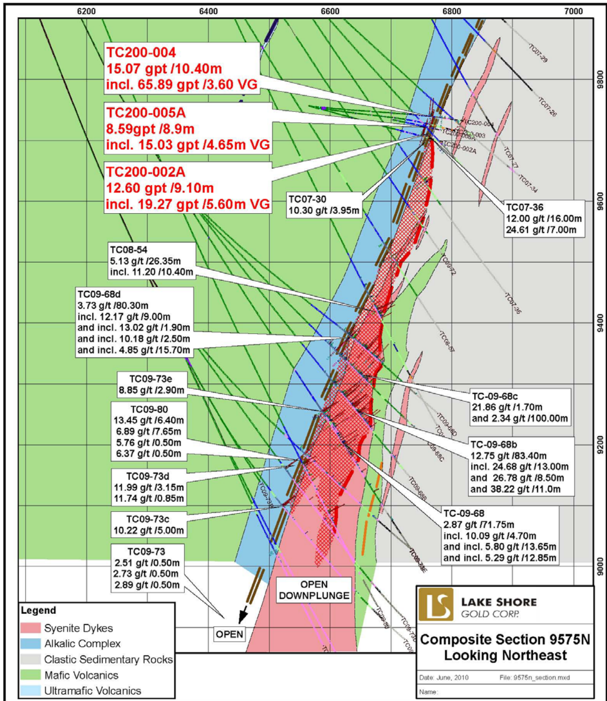
Figure 2. Cross Section
