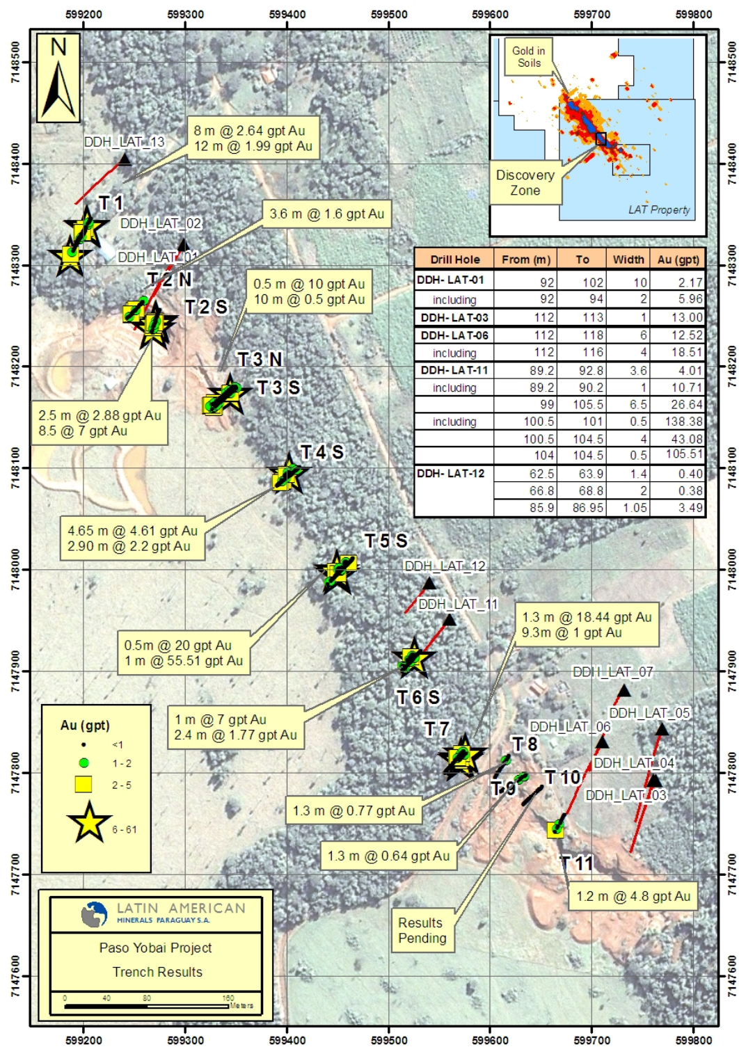
Figure 1: Trenching and drilling compilation map of the northern part of the Discovery Zone.
