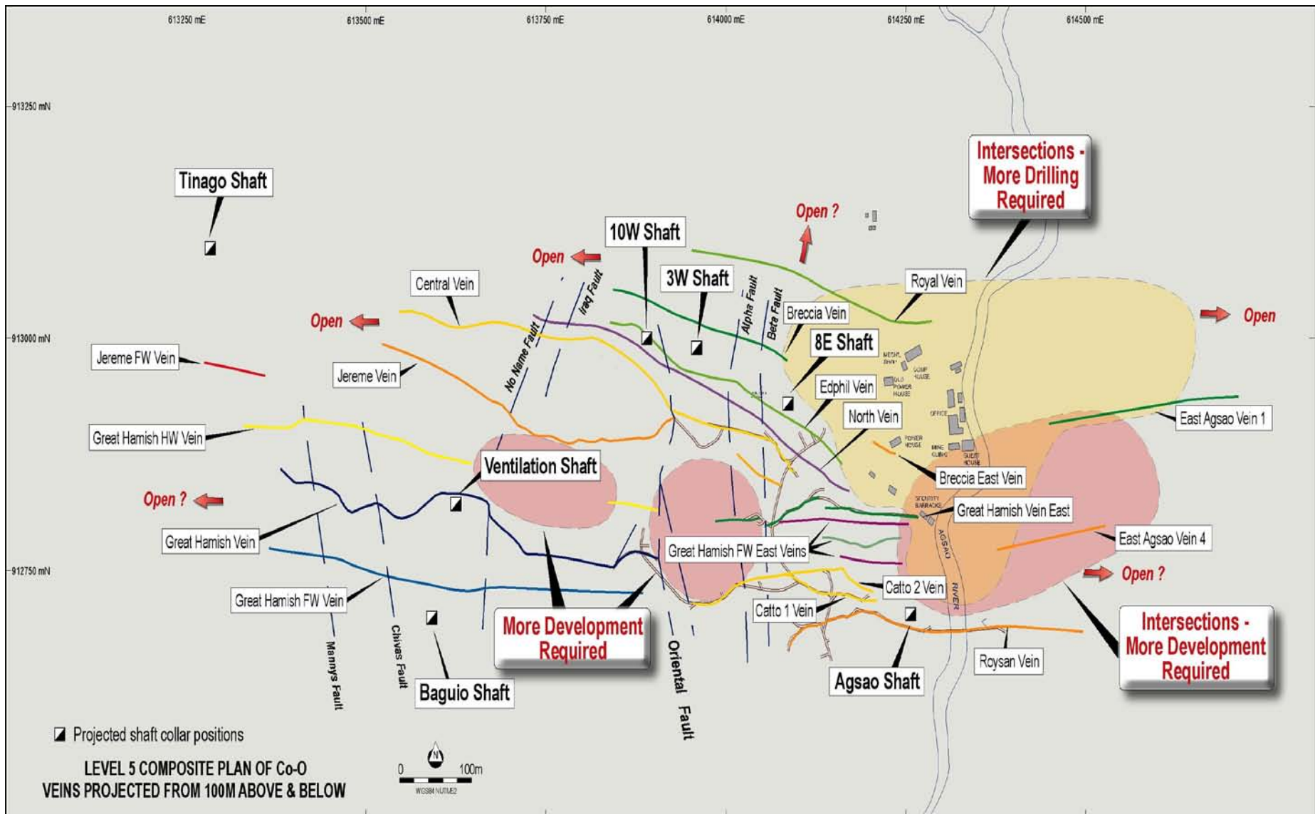
Figure 2. Co-O Mine composite map showing vein and workings projections to Level 5.
