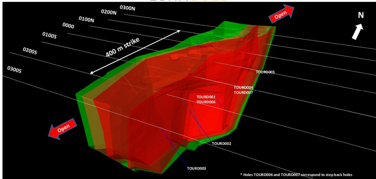
Figure 2. Touro target preliminary 3D geologic model showing main NNE-trending mineralized zone (red) and host tonalities (yellow) and diorites (green).
