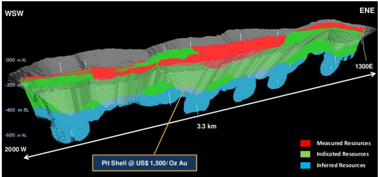
Figure 1. Piaba deposit showing updated resource blocks, new drill holes and new pit shell.
