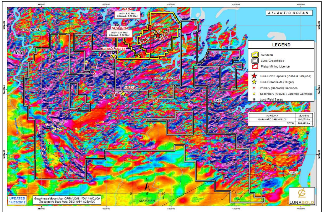
Figure 1. Location of the Ceara and Arete targets, Luna Greenfields project overlain on 1VD magnetic grid (CPRM, 2008).
