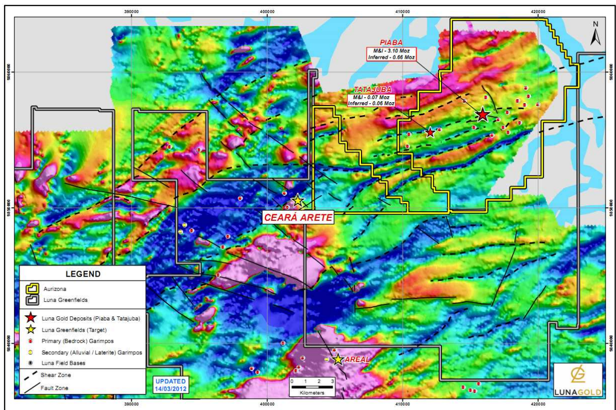
Figure 2. Location of the Ceara and Arete targets within the CASZ – extension of Aurizona mineralized structures into Luna Greenfields. Overlain on total field magnetic grid.
