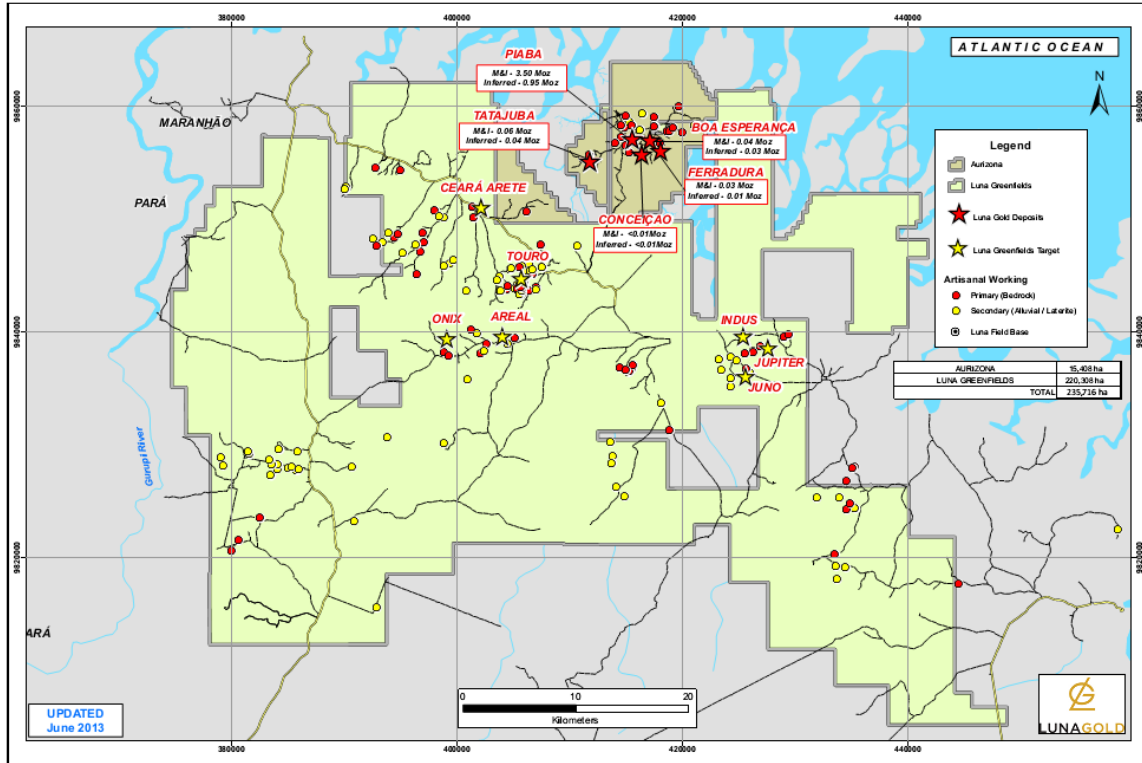
Figure 1. Location of the Jupiter, Indus and Juno targets, Luna Greenfields project overlain on 1VD magnetic grid (CPRM, 2008).
