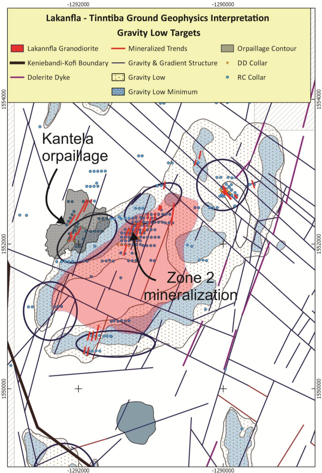
Figure 1: Lakanfla Gravity Compilation
